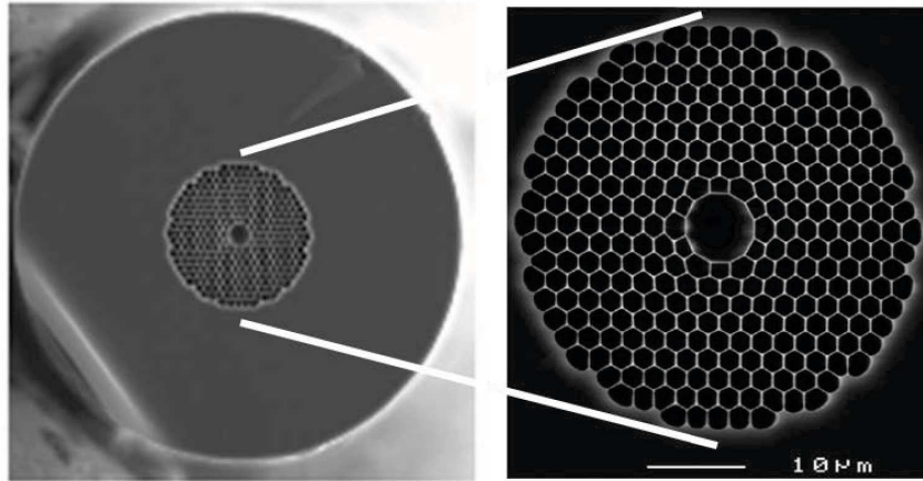
Fig. 1. Hollow-core photonic-bandgap fiber. The diameter of the inner hole, where the atoms are trapped, is 6\ \mu\text{m} . The mode waist inside the fiber is 1.9(2)\ \mu\text{m} . A 3 cm long, vertically mounted piece of fiber is used for the experiments.
