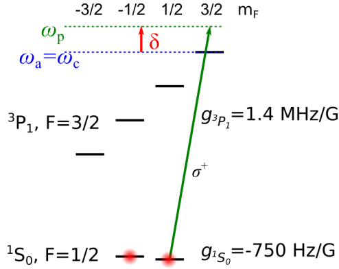
FIG. 3. Hyperfine structure of the 6s^2 1S_0 state and the 6s6p^3P_1 state relevant to phase-shift measurement: the F = 1/2 manifold of the 6s6p^3P_1 state is -6 GHz detuned from the F = 3/2 manifold and therefore is not drawn in the figure. g_{3P_1} and g_{1S_0} are g factors for the 6s6p^3P_1 state and the s^2 1S_0 state, respectively. \omega_a , \omega_c , and \omega_p are the frequencies of the s^2 1S_0 \rightarrow 6s6p^3P_1 atomic transition, the cavity resonance, and the probing laser, respectively.
